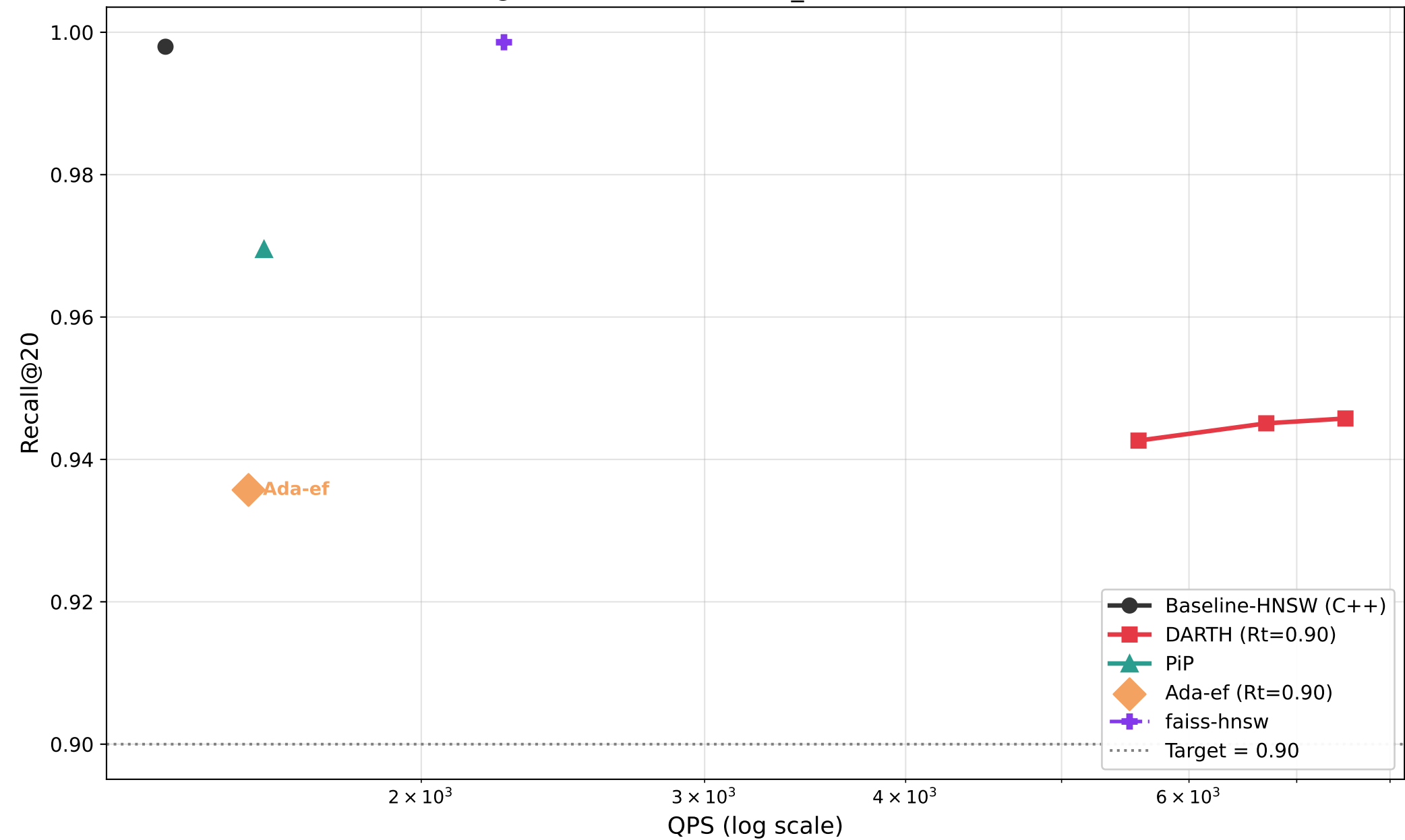
Recall@20 vs QPS — fashion_mnist (M=8, efC=200)
