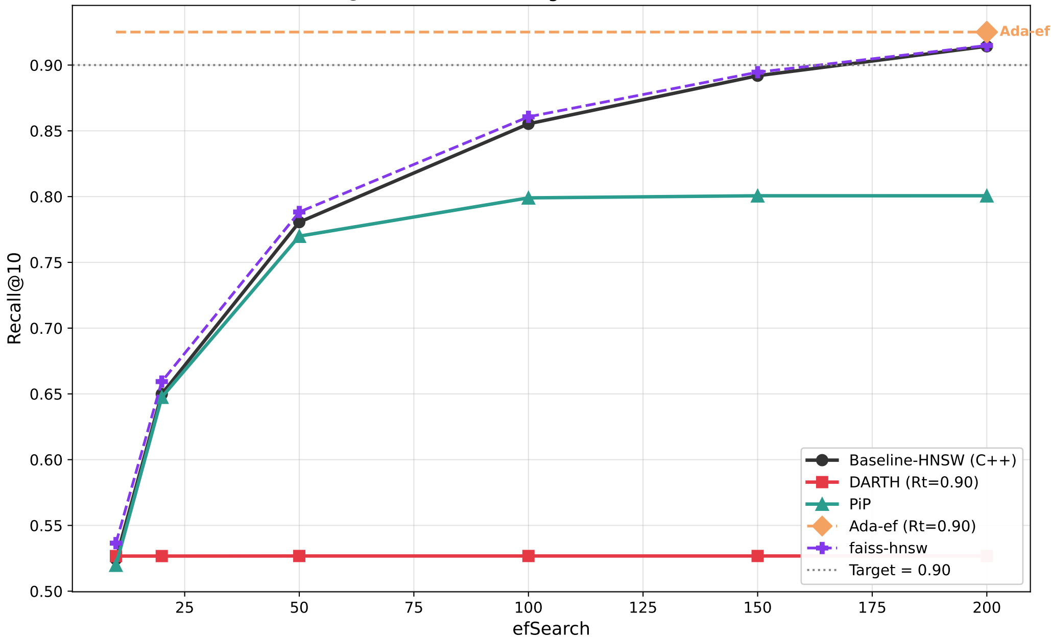
Recall@10 vs efSearch — glove100 (M=16, efC=128)
