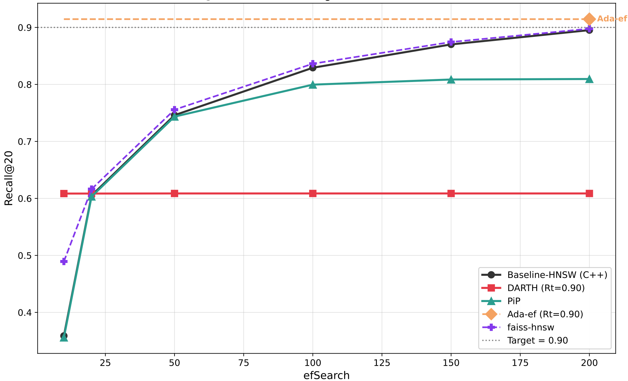
Recall@20 vs efSearch — glove100 (M=16, efC=128)
