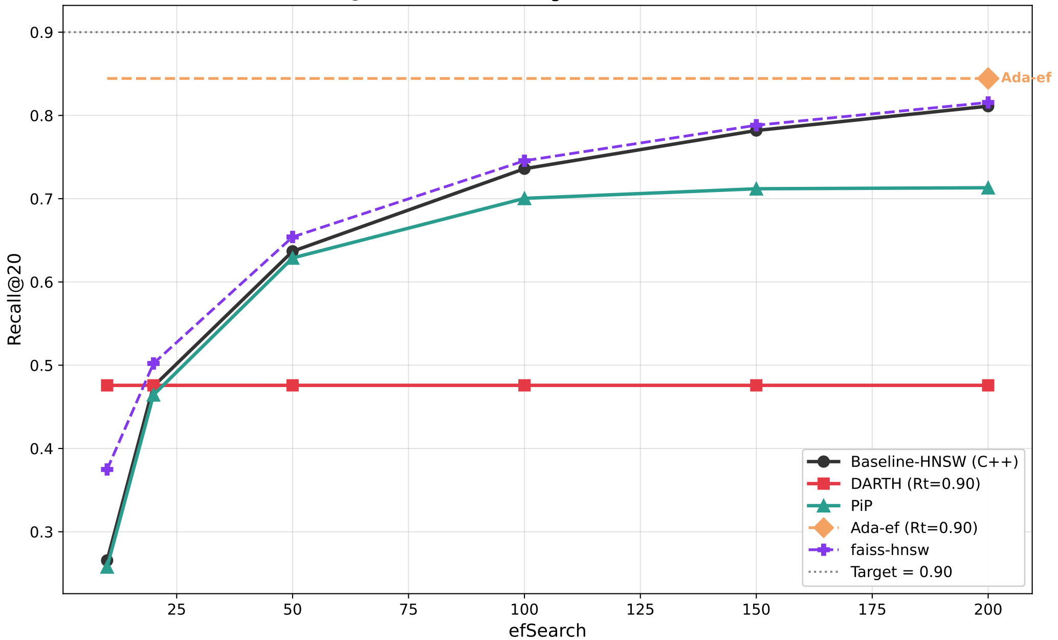
Recall@20 vs efSearch — glove100 (M=8, efC=128)
