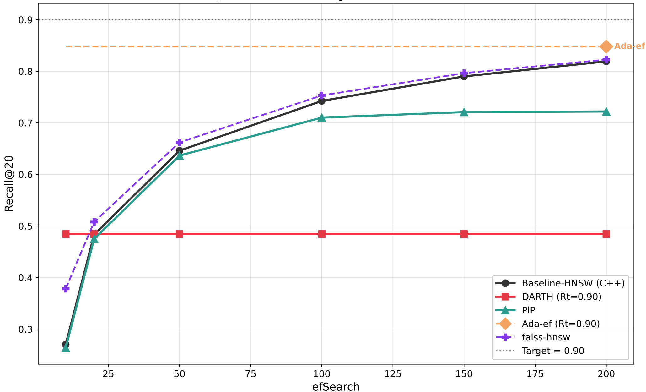
Recall@20 vs efSearch — glove100 (M=8, efC=200)
