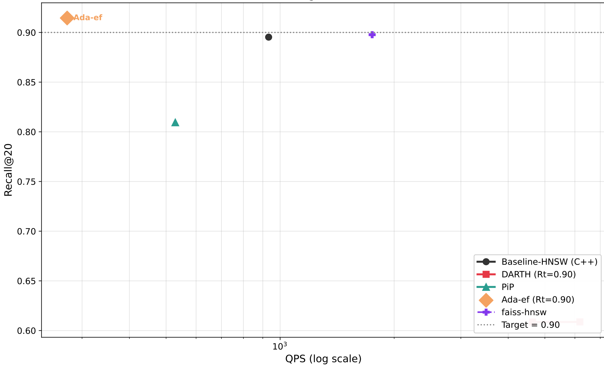
Recall@20 vs QPS — glove100 (M=16, efC=128)
