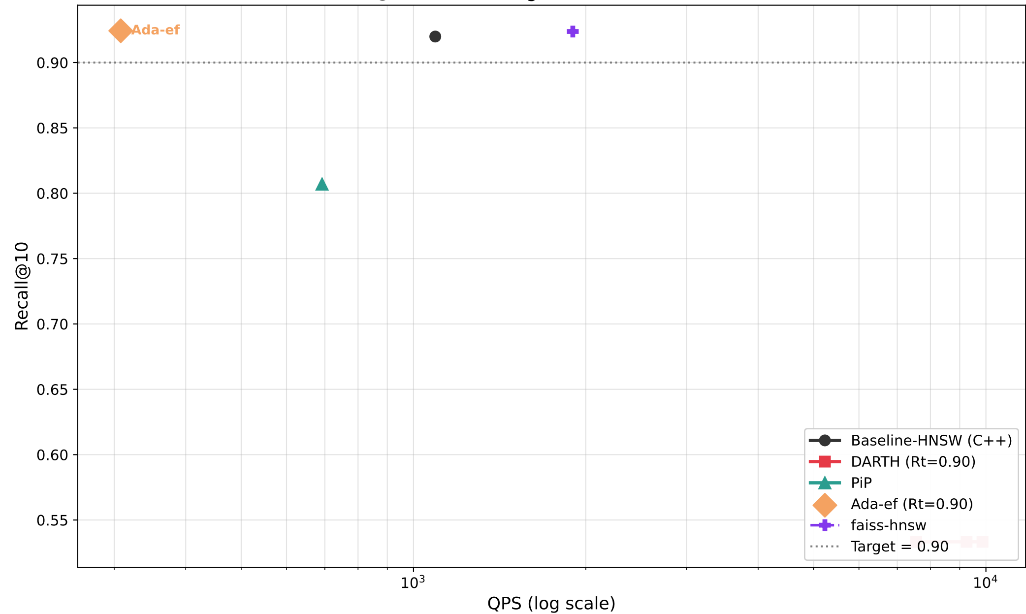
Recall@10 vs QPS — glove100 (M=16, efC=200)
