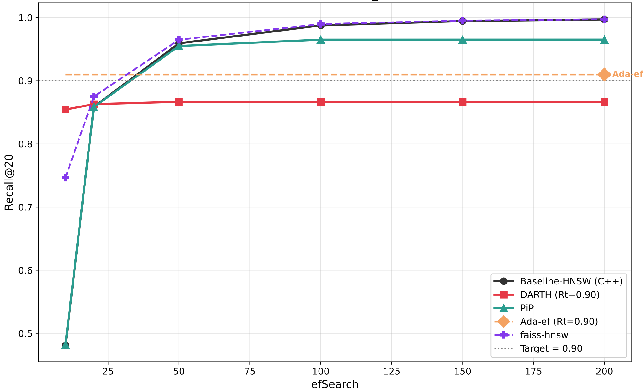
Recall@20 vs efSearch — msmarco_text (M=16, efC=128)
