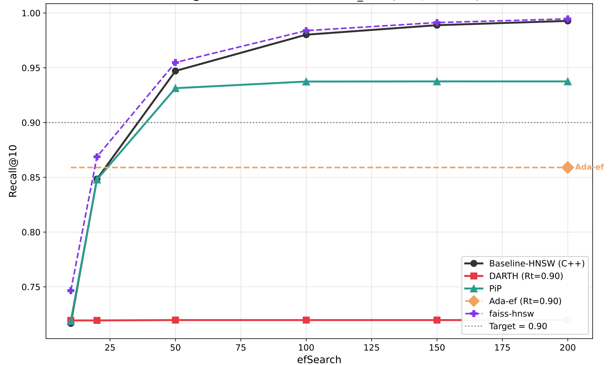
Recall@10 vs efSearch — msmarco_text (M=8, efC=128)
