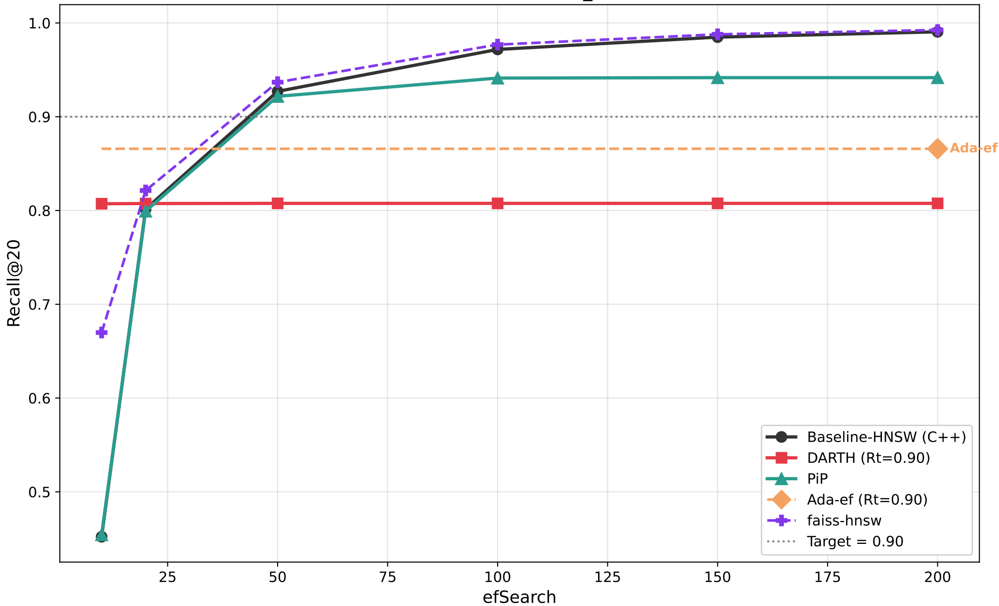
Recall@20 vs efSearch — msmarco_text (M=8, efC=128)
