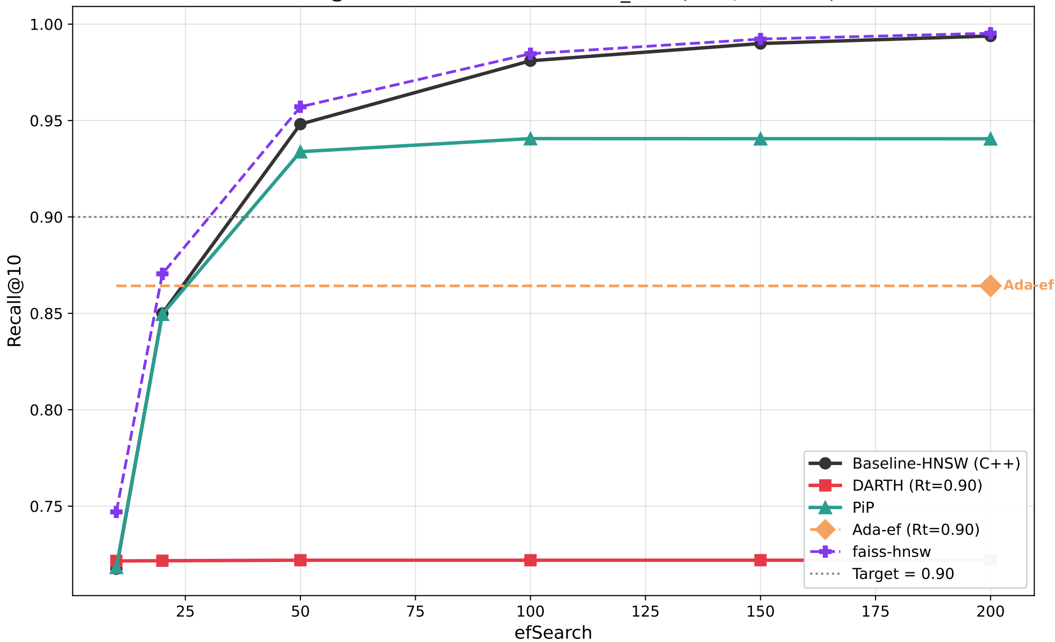
Recall@10 vs efSearch — msmarco_text (M=8, efC=200)
