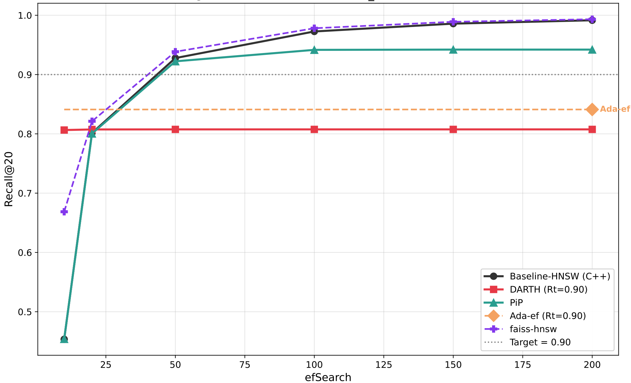
Recall@20 vs efSearch — msmarco_text (M=8, efC=200)
