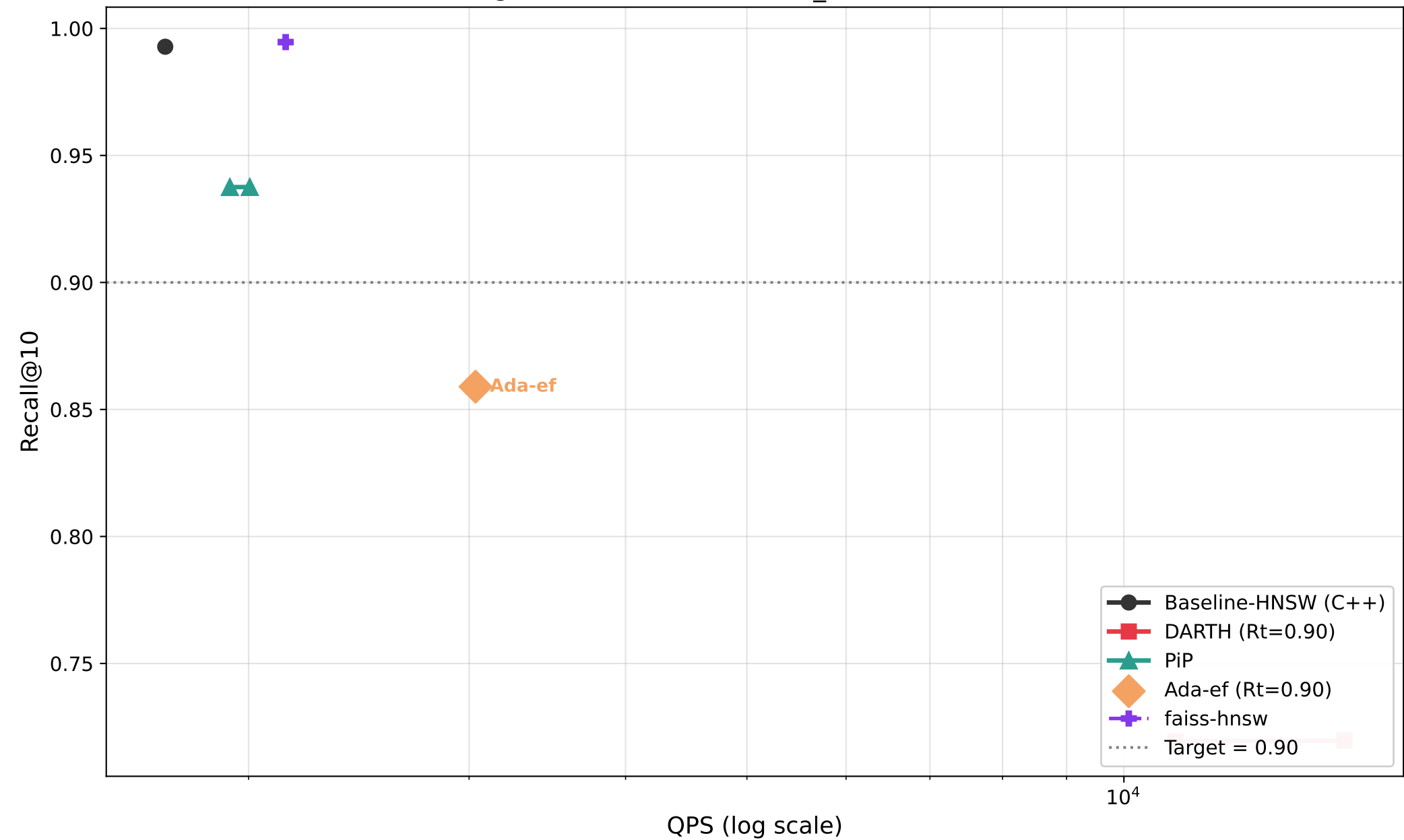
Recall@10 vs QPS — msmarco_text (M=8, efC=128)
