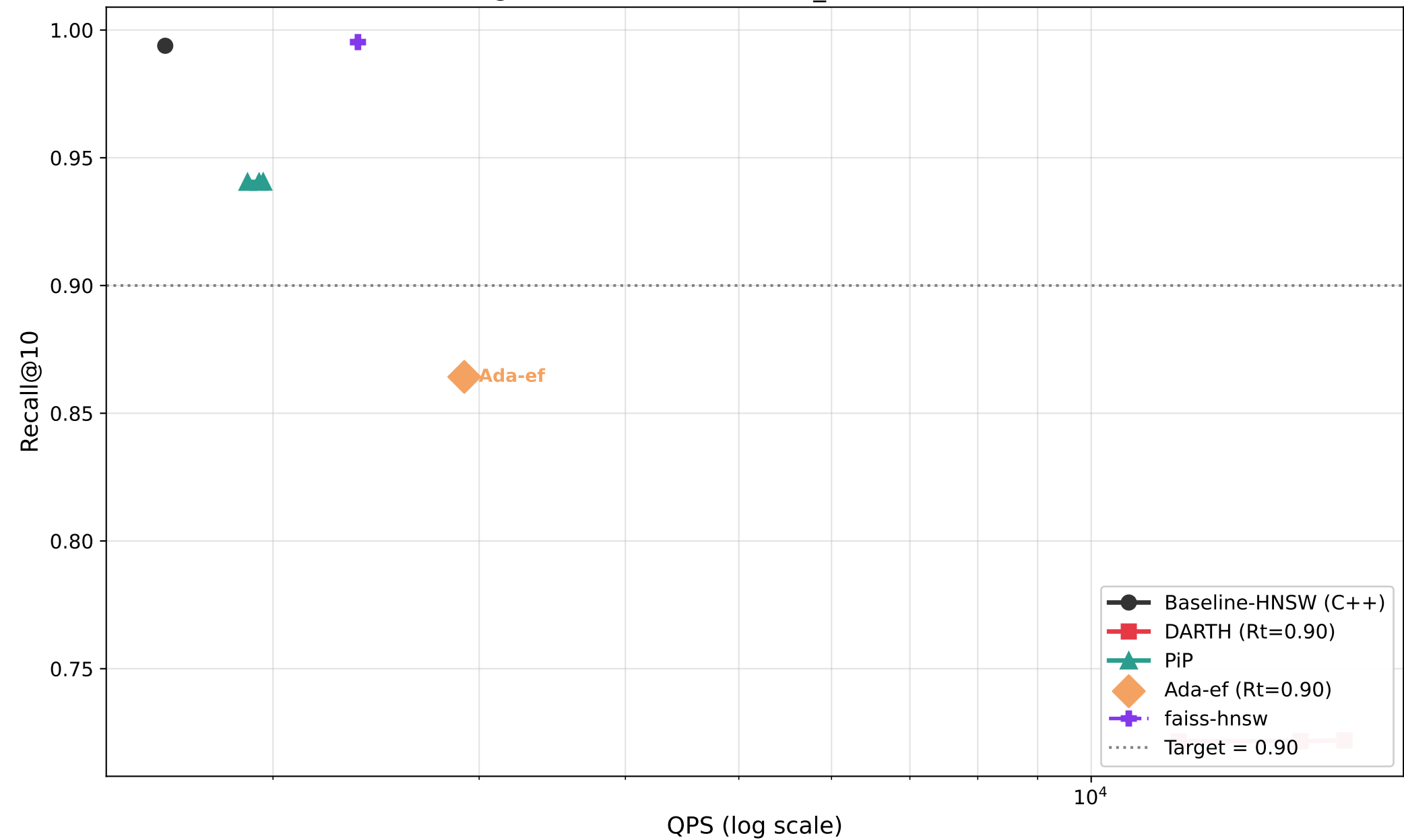
Recall@10 vs QPS — msmarco_text (M=8, efC=200)
