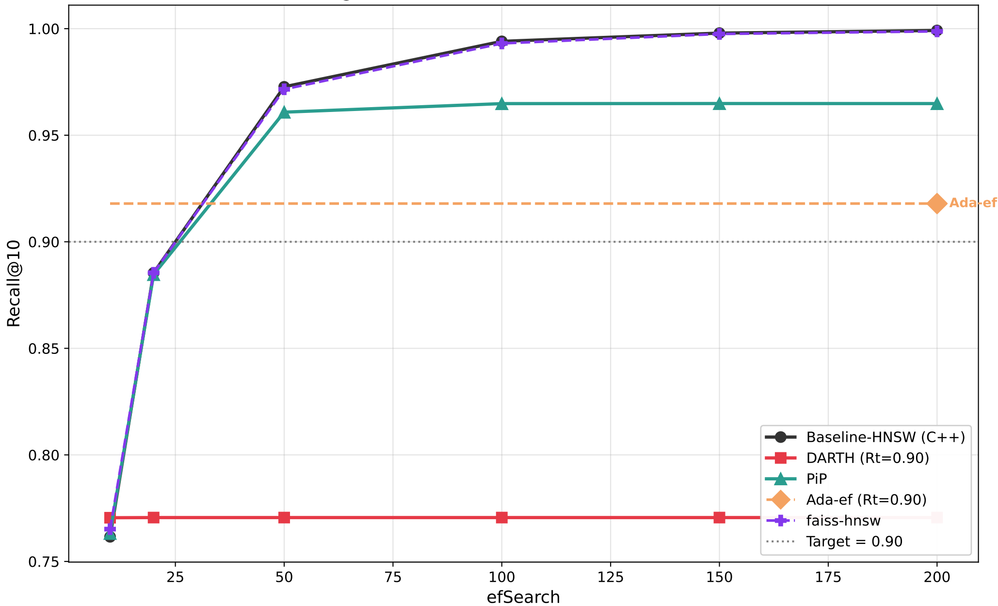
Recall@10 vs efSearch — sift128 (M=16, efC=128)
