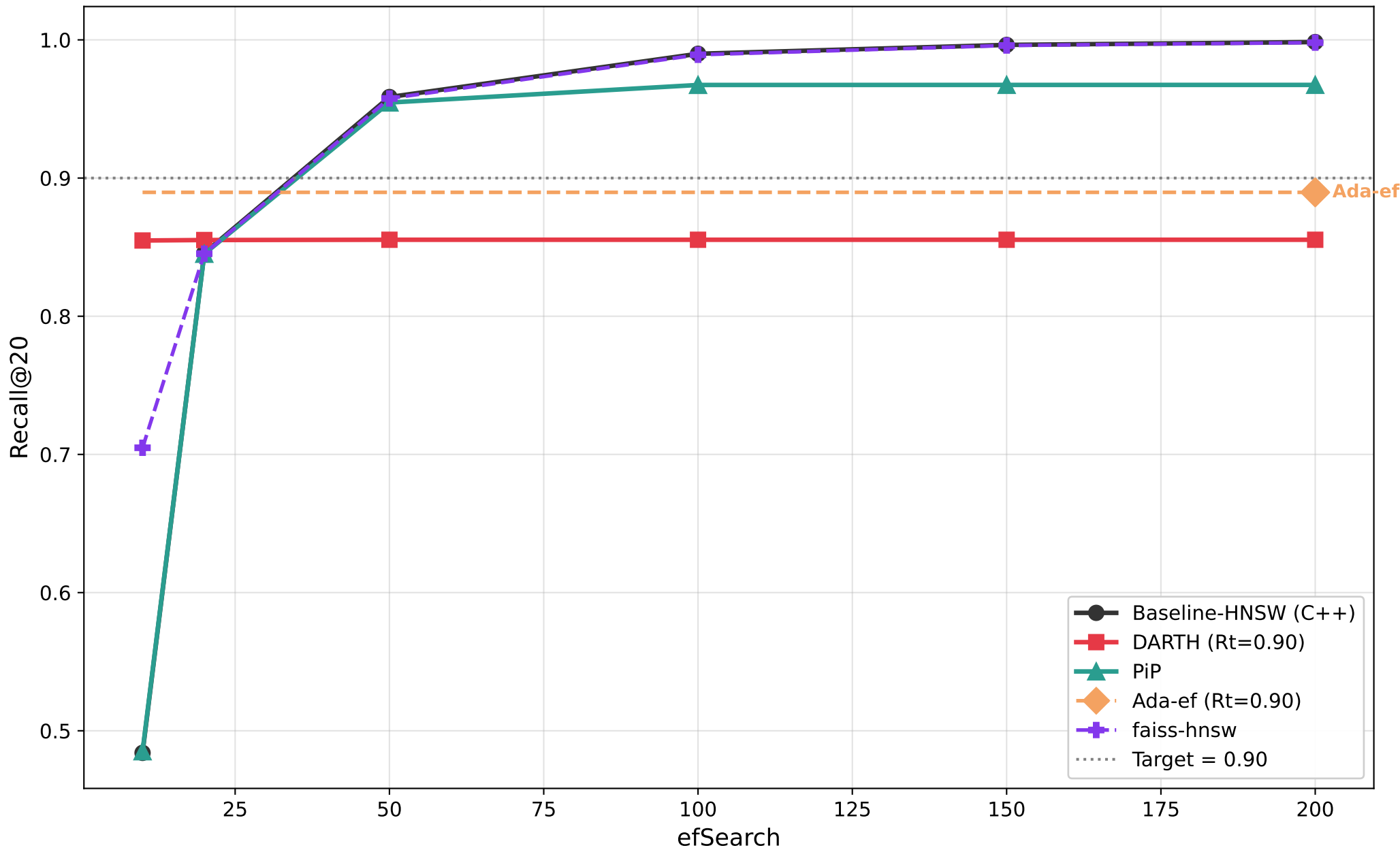
Recall@20 vs efSearch — sift128 (M=16, efC=128)
