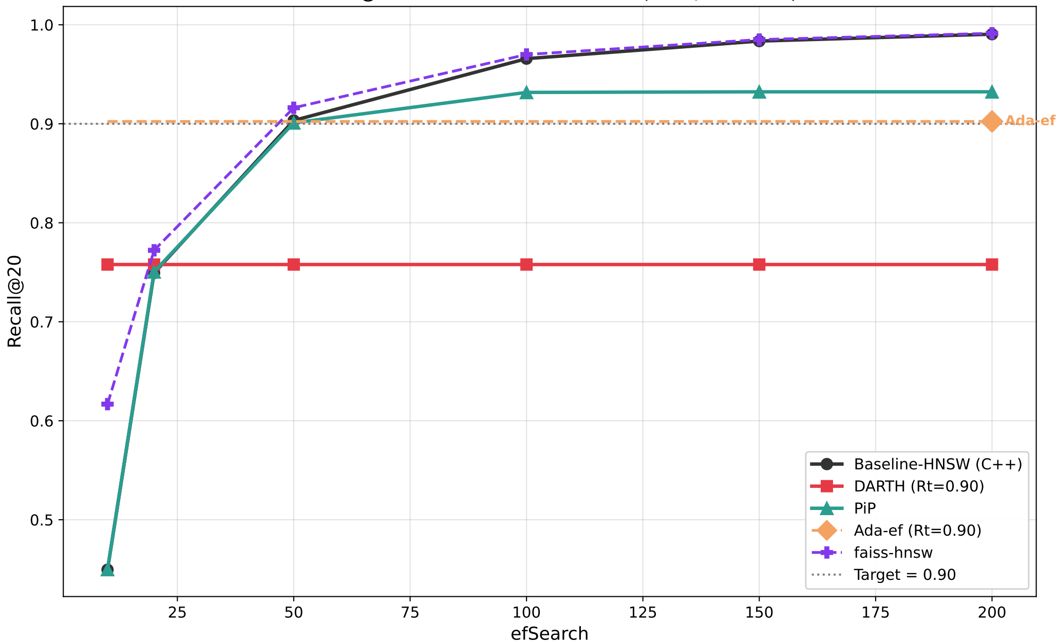
Recall@20 vs efSearch — sift128 (M=8, efC=128)
