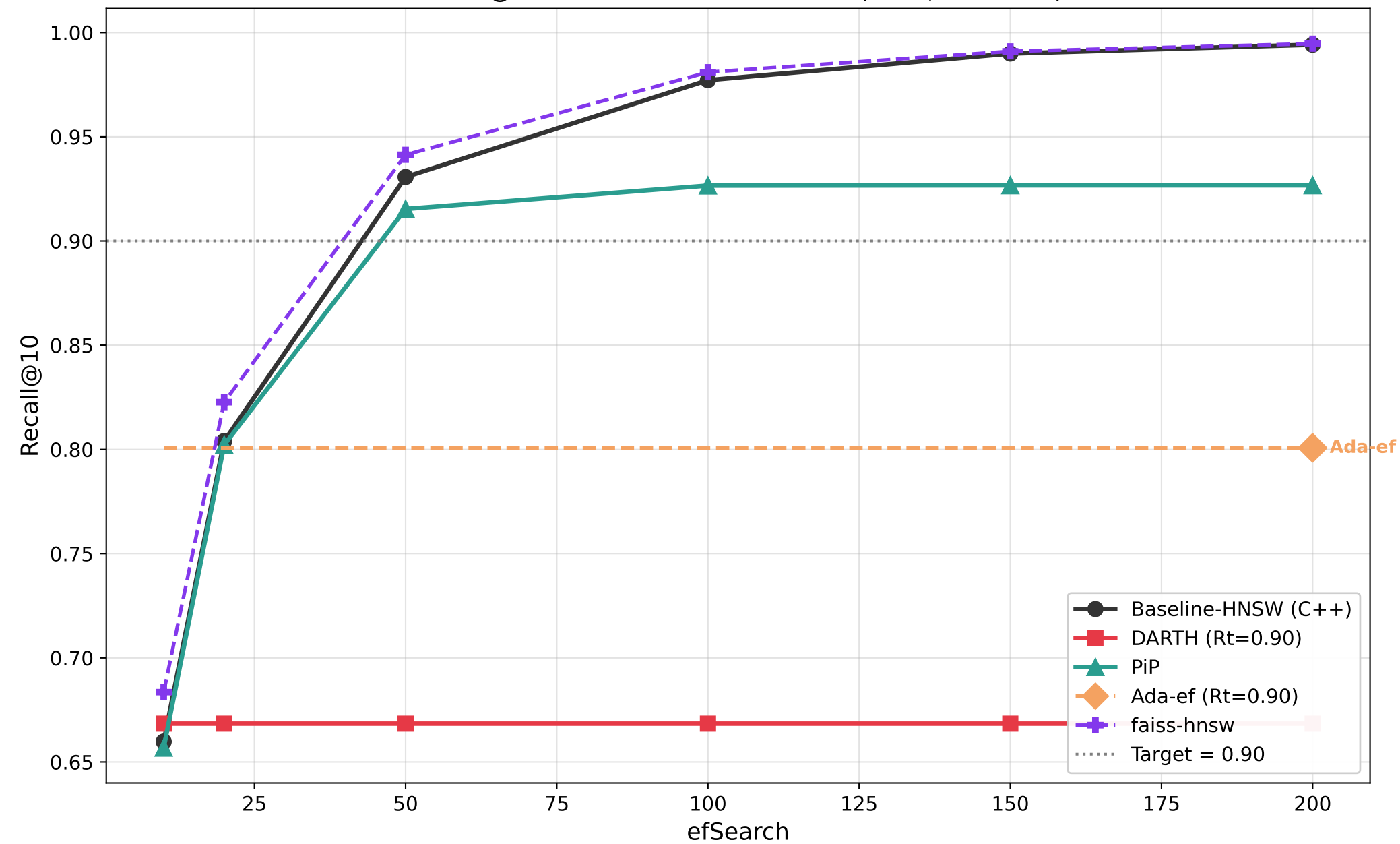
Recall@10 vs efSearch — sift128 (M=8, efC=200)
