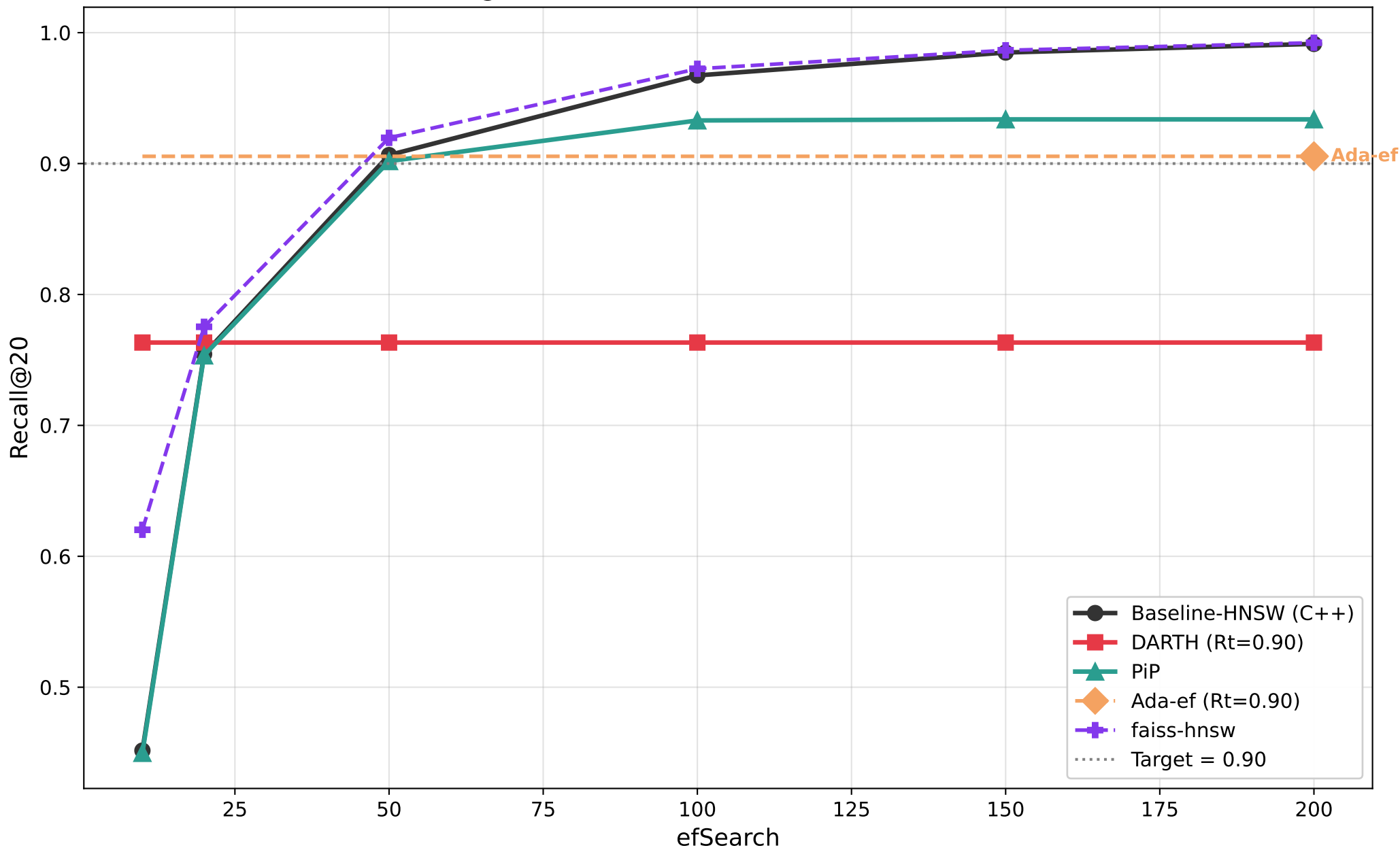
Recall@20 vs efSearch — sift128 (M=8, efC=200)
