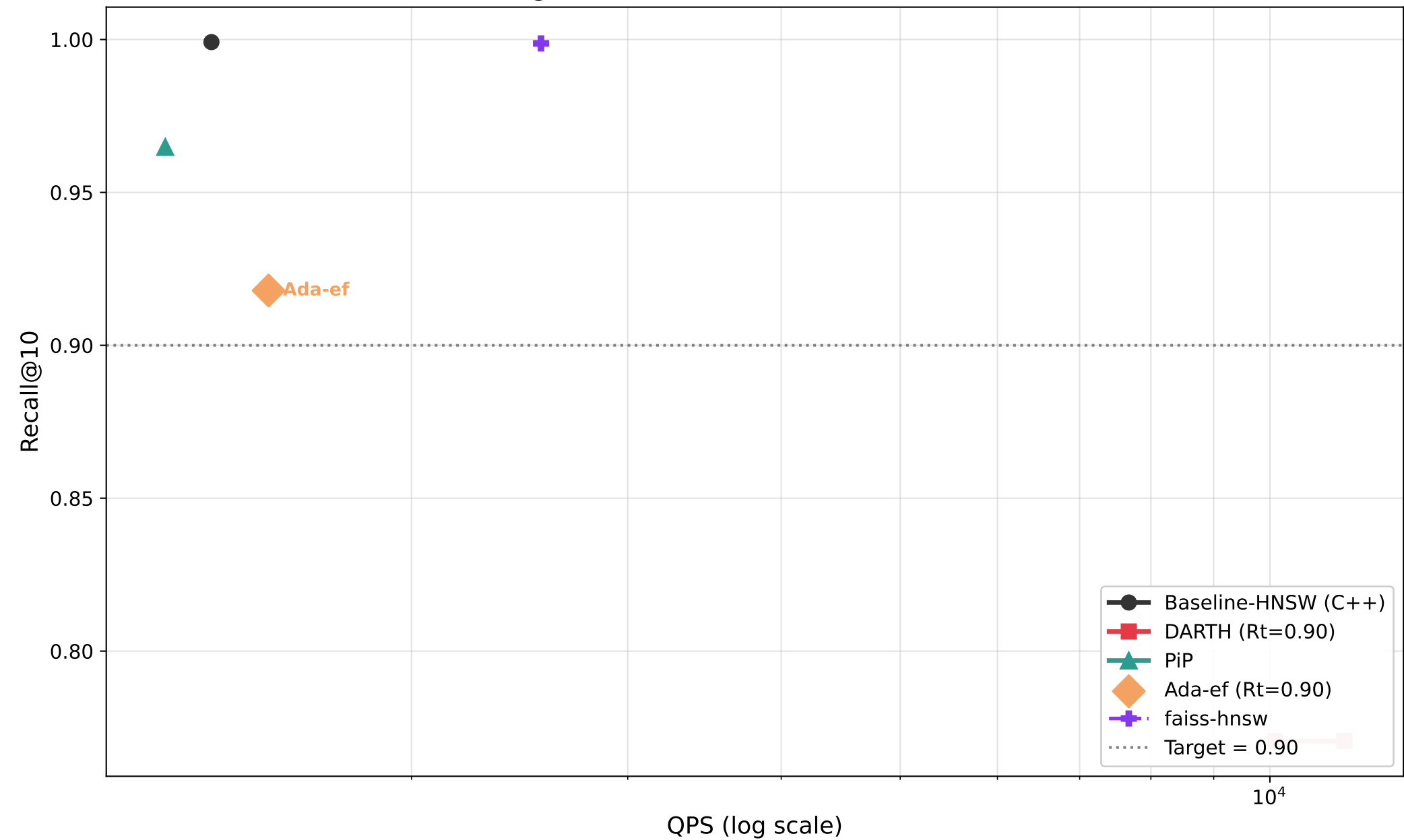
Recall@10 vs QPS — sift128 (M=16, efC=128)
