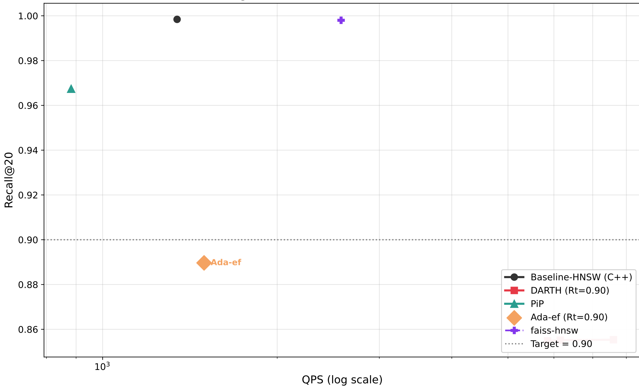
Recall@20 vs QPS — sift128 (M=16, efC=128)
