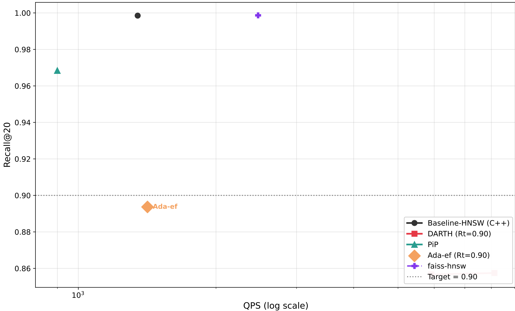
Recall@20 vs QPS — sift128 (M=16, efC=200)
