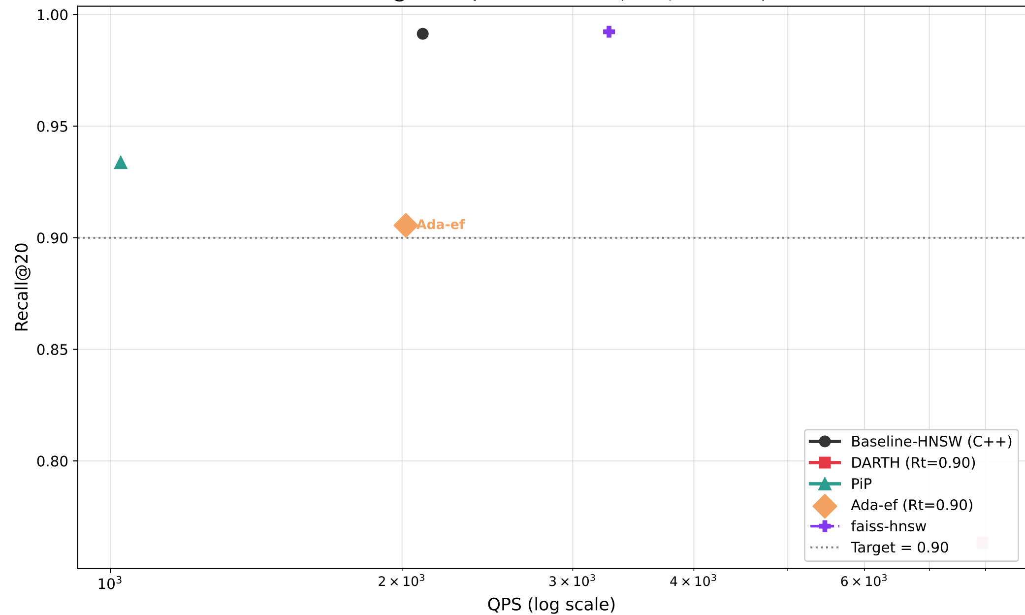
Recall@20 vs QPS — sift128 (M=8, efC=200)
