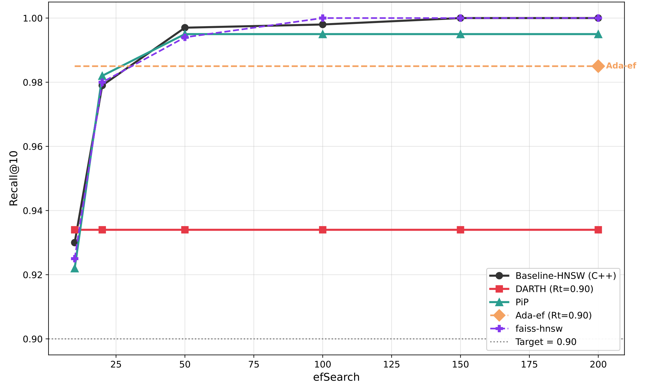
Recall@10 vs efSearch — siftsmall (M=16, efC=200)
