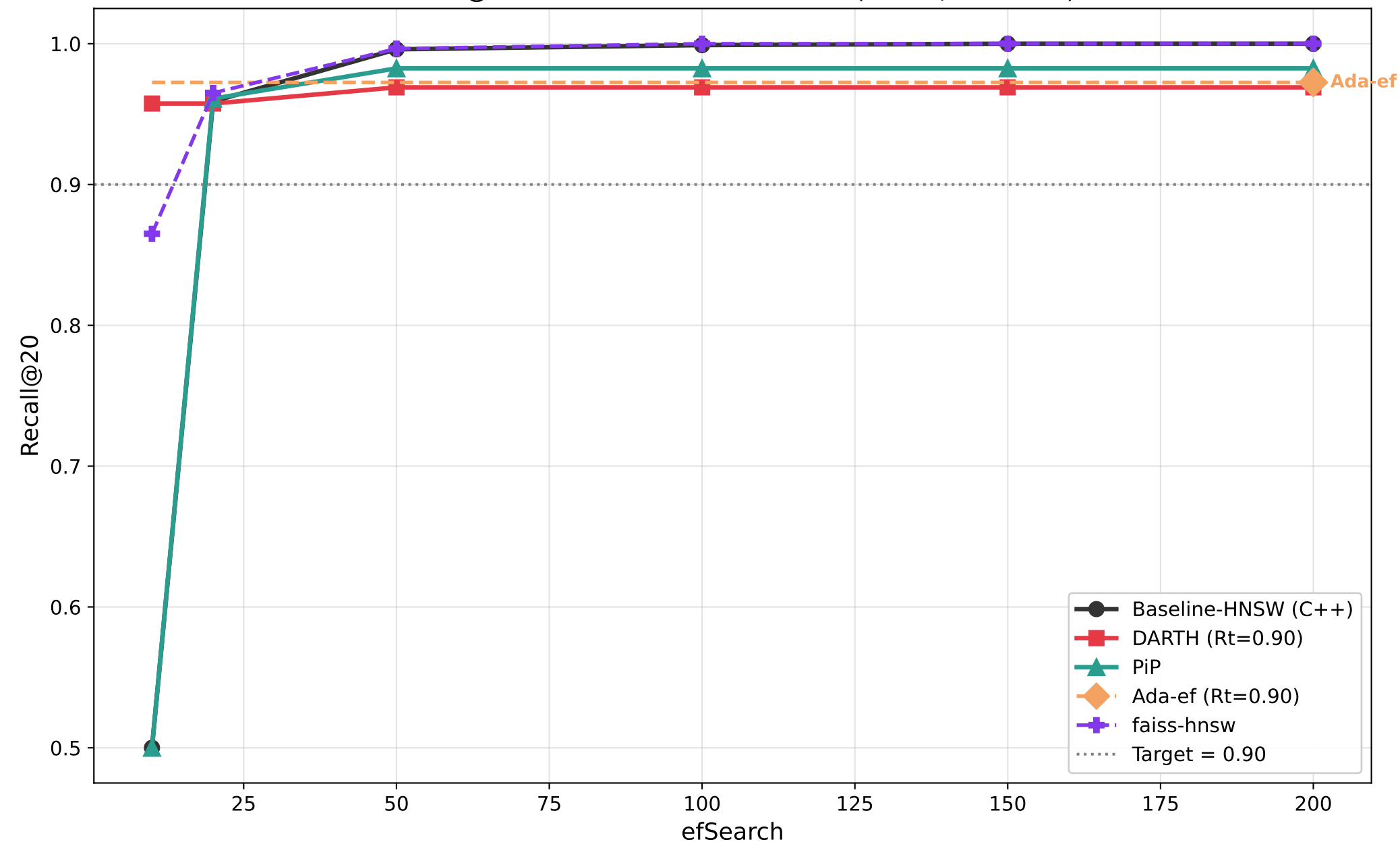
Recall@20 vs efSearch — siftsmall (M=16, efC=200)
