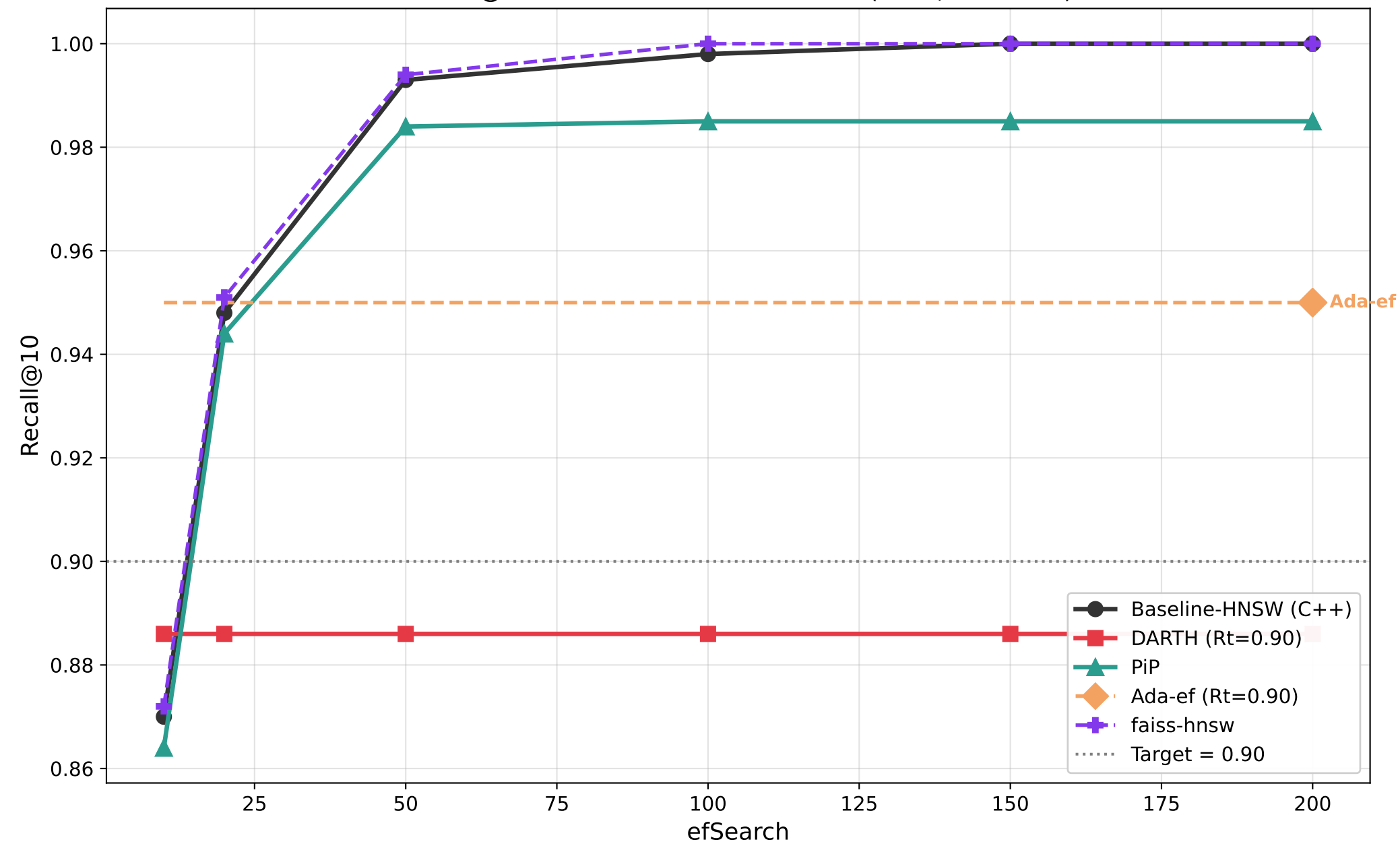
Recall@10 vs efSearch — siftsmall (M=8, efC=128)
