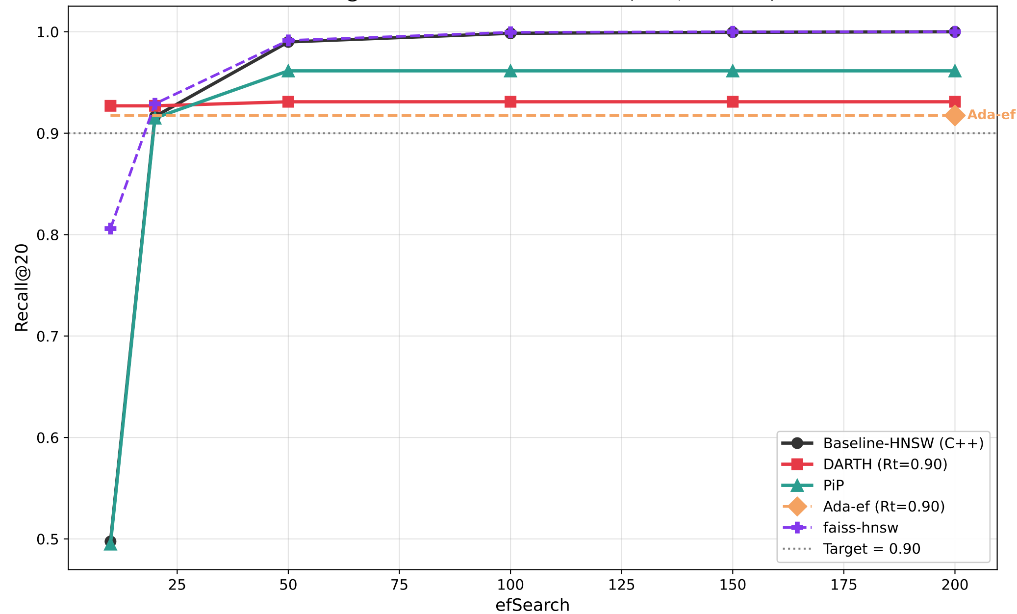
Recall@20 vs efSearch — siftsmall (M=8, efC=128)
