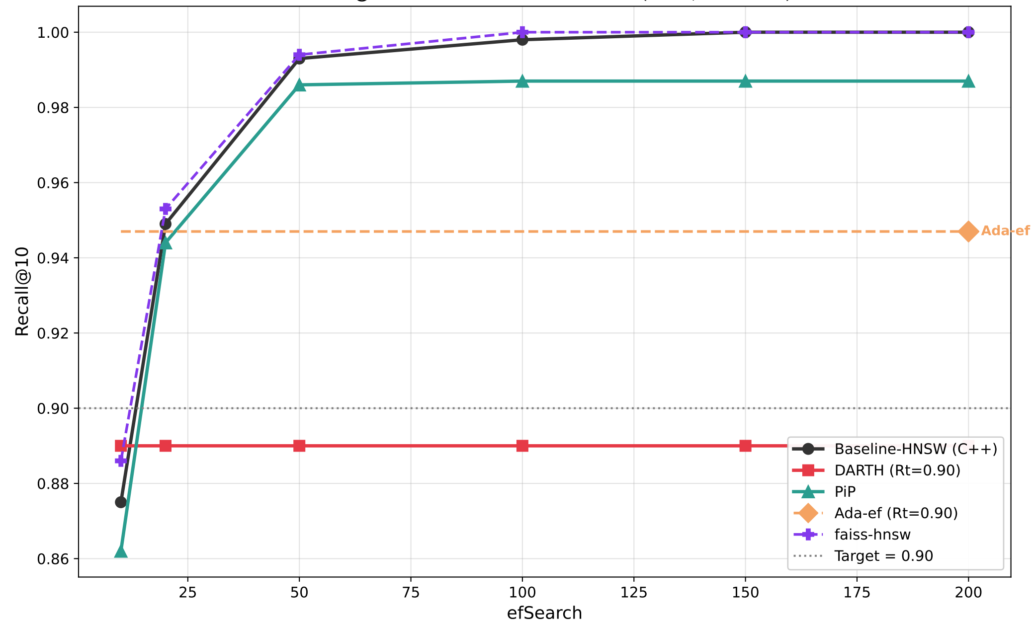
Recall@10 vs efSearch — siftsmall (M=8, efC=200)
