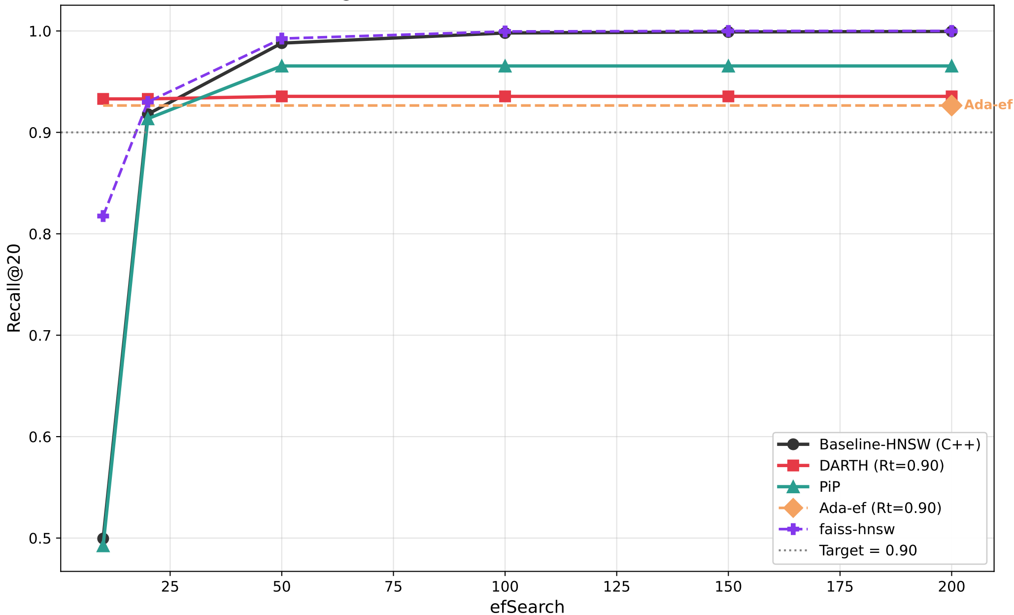
Recall@20 vs efSearch — siftsmall (M=8, efC=200)
