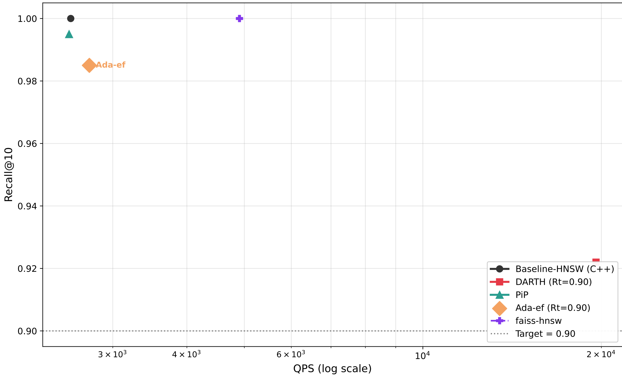
Recall@10 vs QPS — siftsmall (M=16, efC=128)
