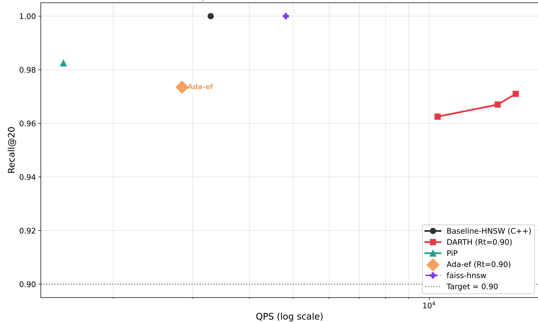
Recall@20 vs QPS — siftsmall (M=16, efC=128)
