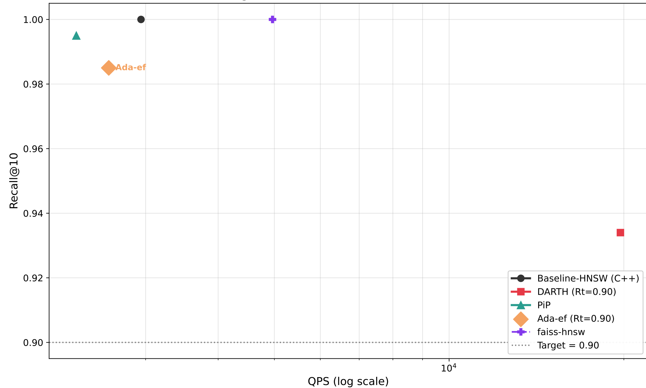
Recall@10 vs QPS — siftsmall (M=16, efC=200)
