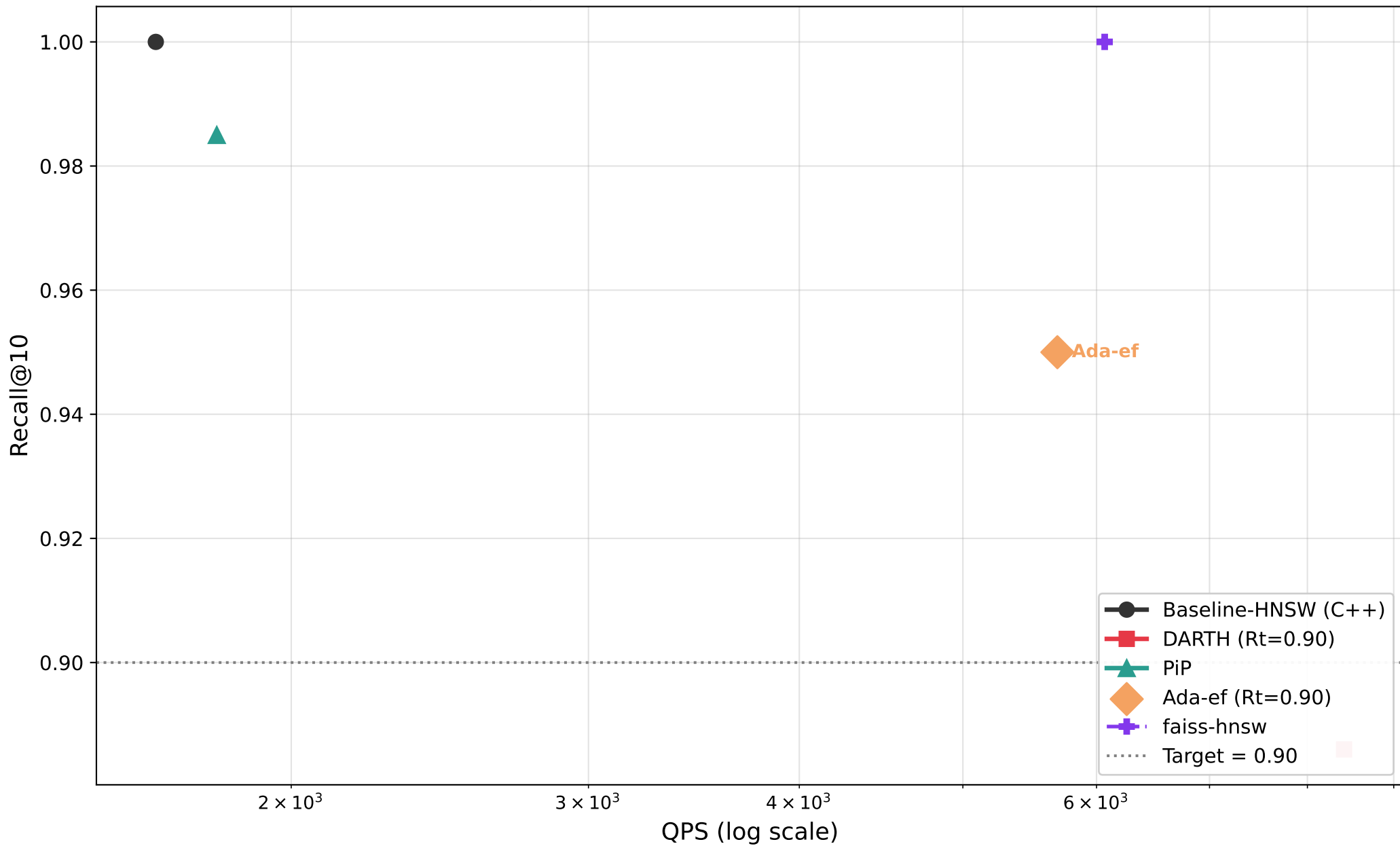
Recall@10 vs QPS — siftsmall (M=8, efC=128)
