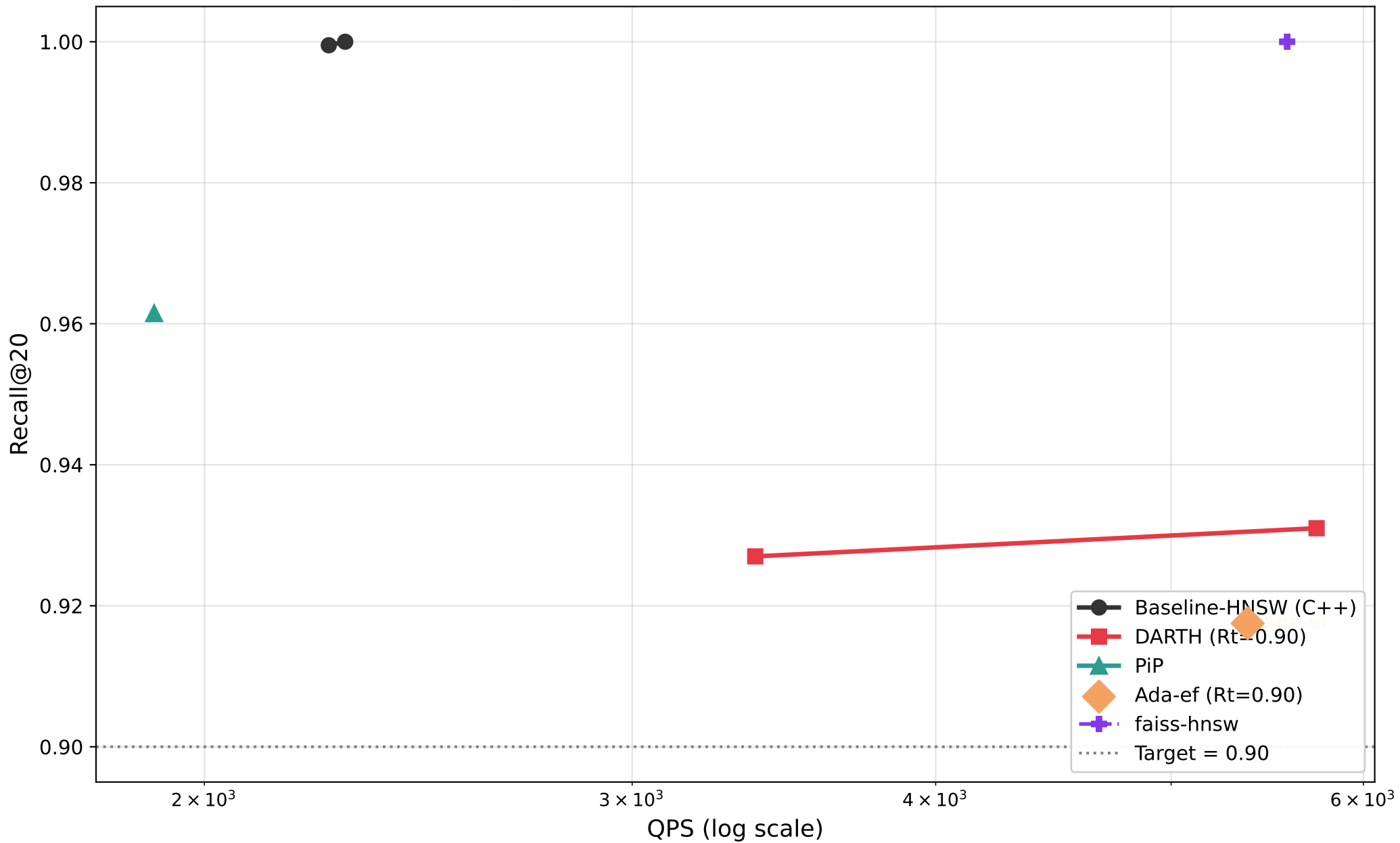
Recall@20 vs QPS — siftsmall (M=8, efC=128)
