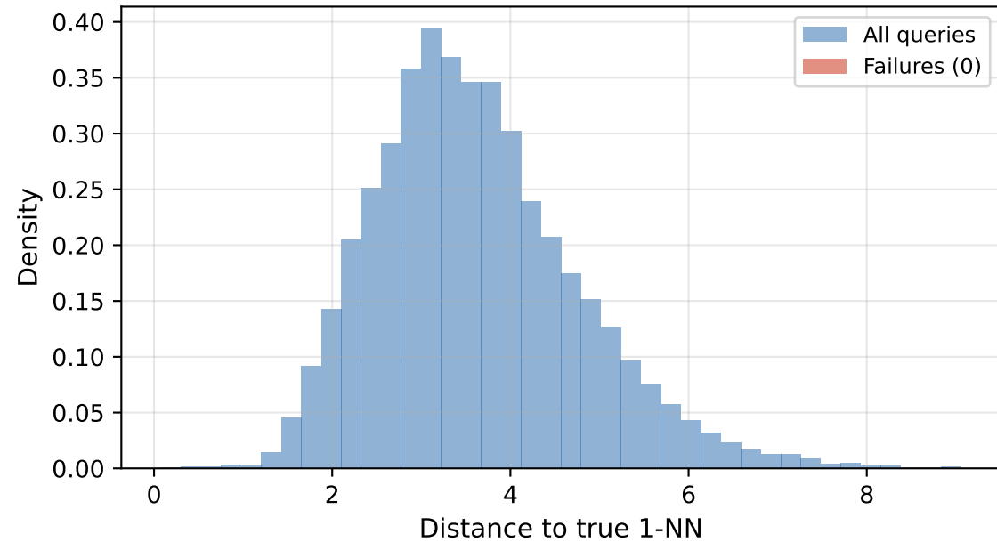
Distance To True 1-Nn
