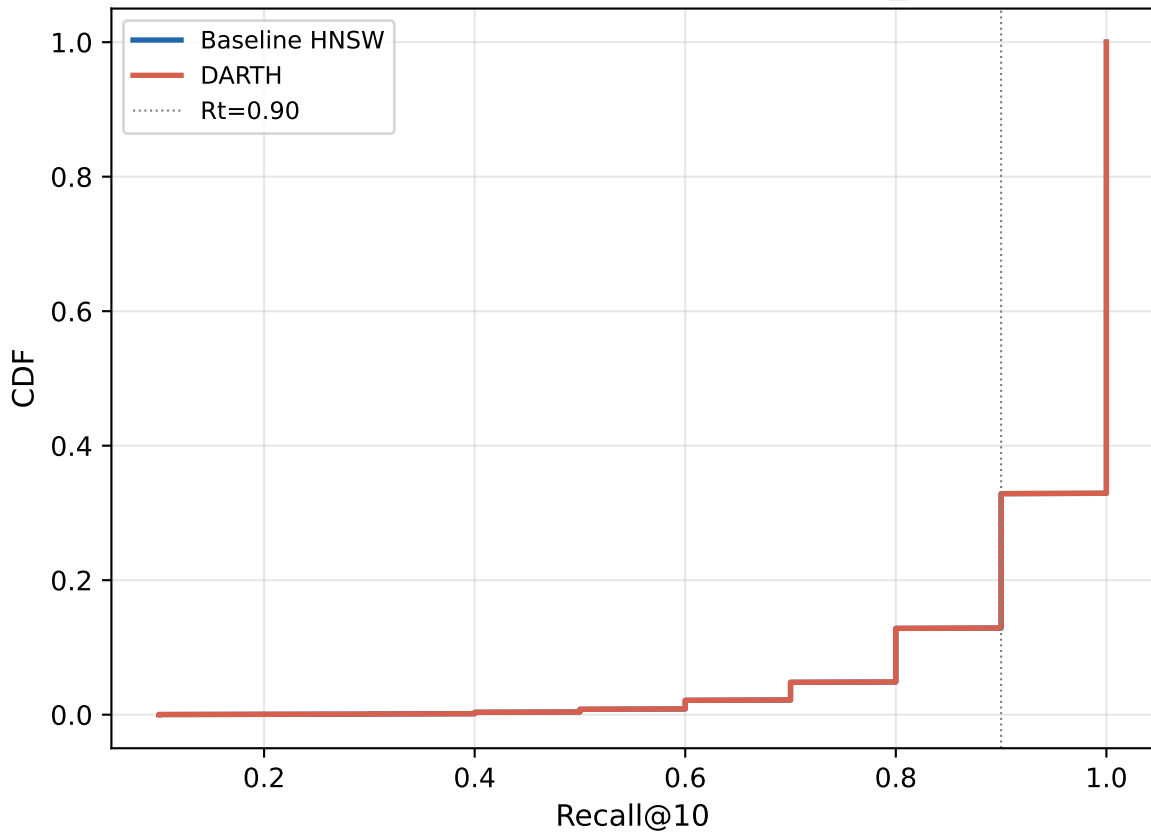
CDF of per-query Recall@10 — fashion_mnist
