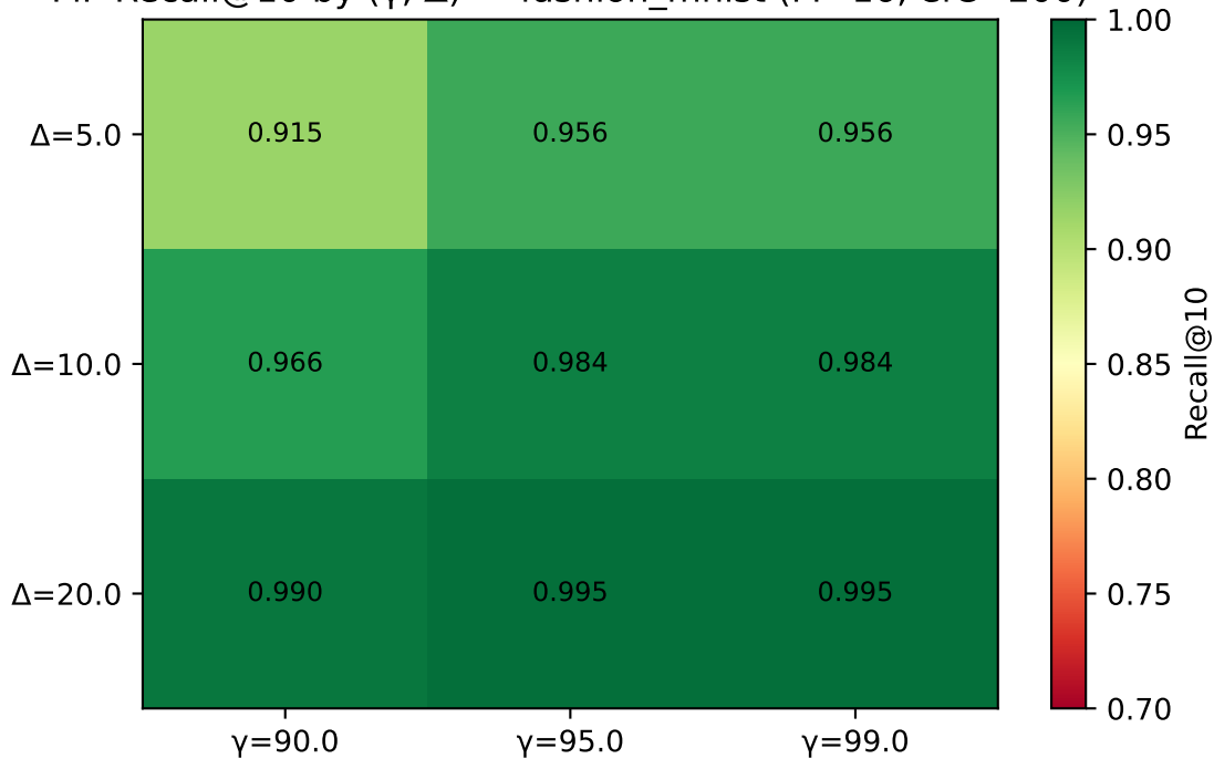
PiP Recall@10 by ( \gamma , \Delta ) — fashion_mnist (M=16, efC=200)
