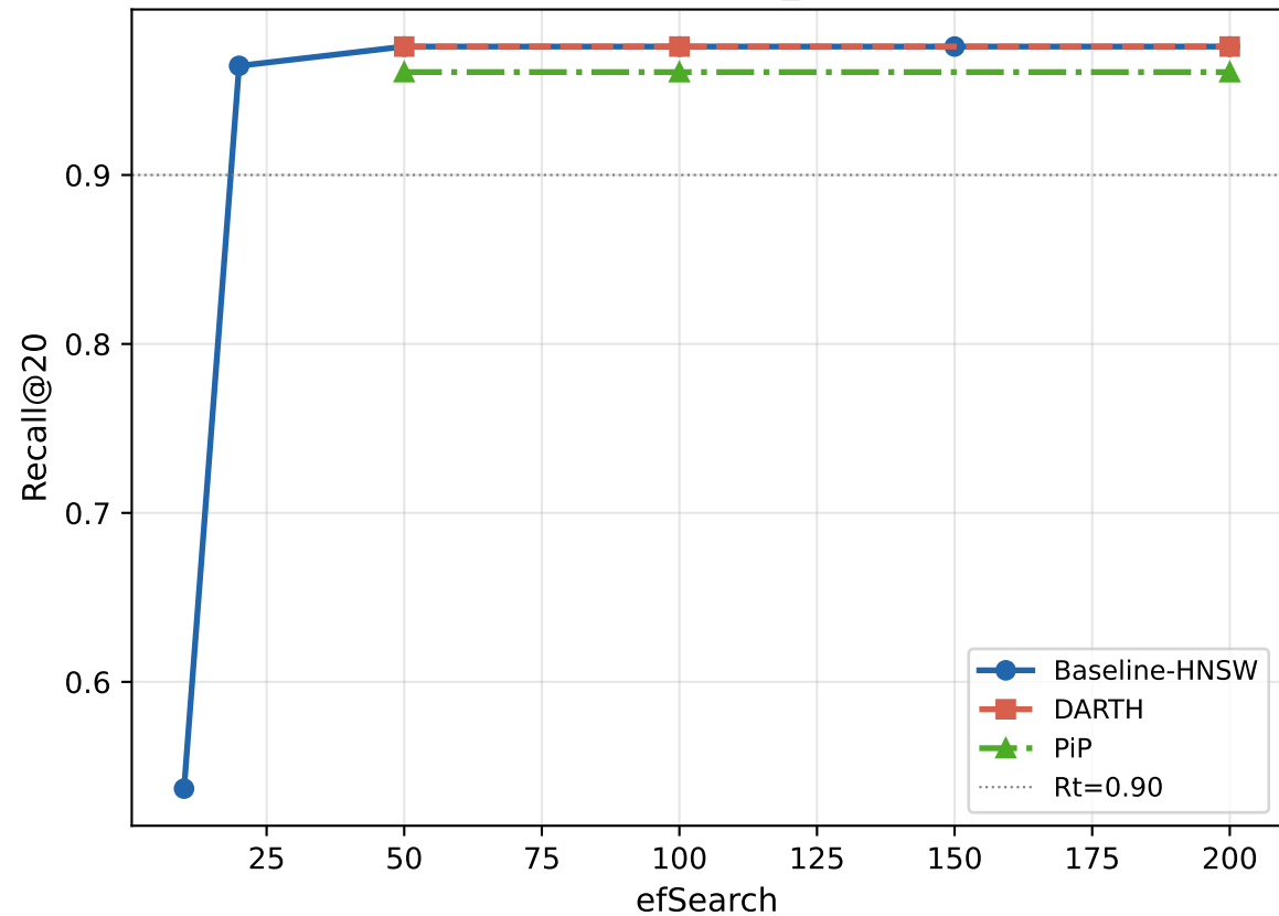
Recall@20 vs efSearch — fashion_mnist (M=16, efC=200)
