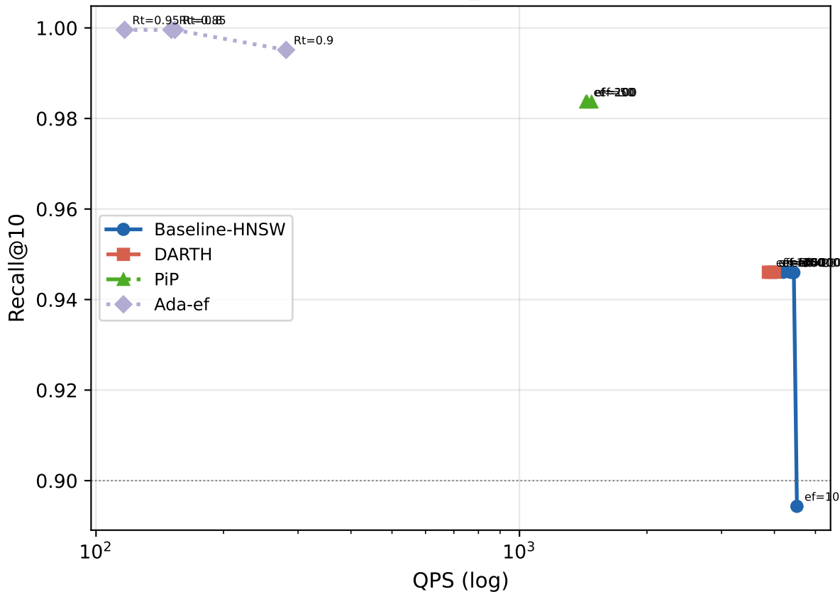
Recall@10-QPS — fashion_mnist (M=16, efC=200)
