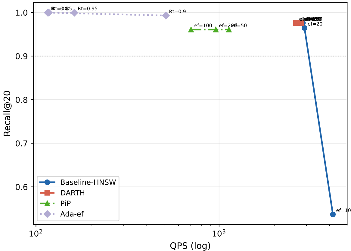
Recall@20-QPS — fashion_mnist (M=16, efC=200)
