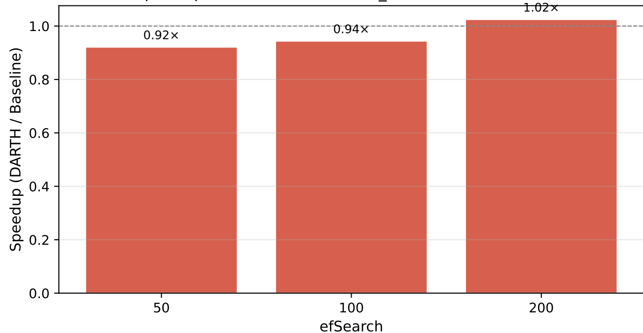
DARTH Speedup at Rt=0.90 — fashion_mnist (M=16, efC=200, k=20)
