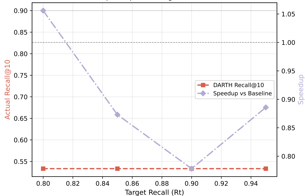
DARTH: Recall & Speedup vs Rt — glove100 (M=16, efC=200)
