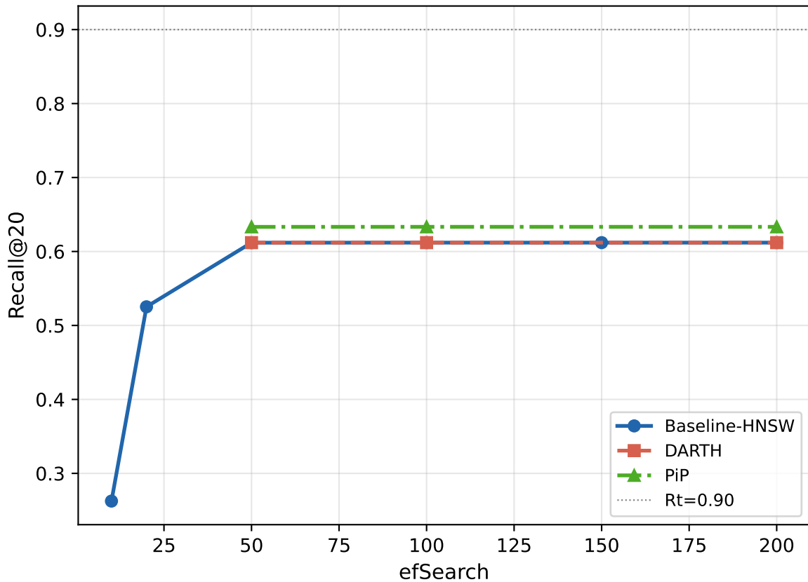
Recall@20 vs efSearch — glove100 (M=16, efC=200)
