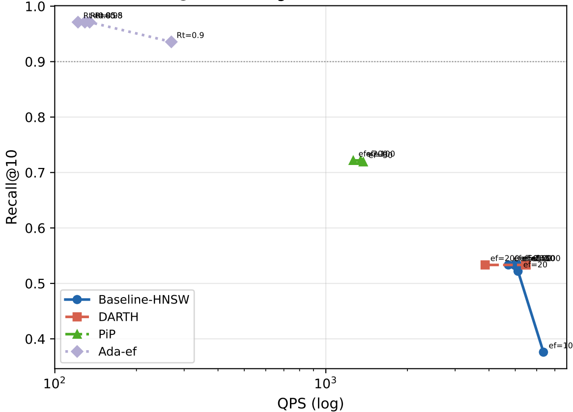
Recall@10-QPS — glove100 (M=16, efC=200)
