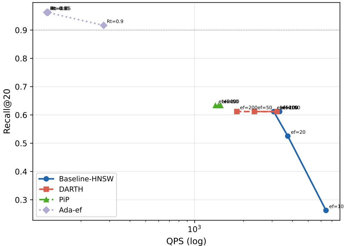
Recall@20-QPS — glove100 (M=16, efC=200)
