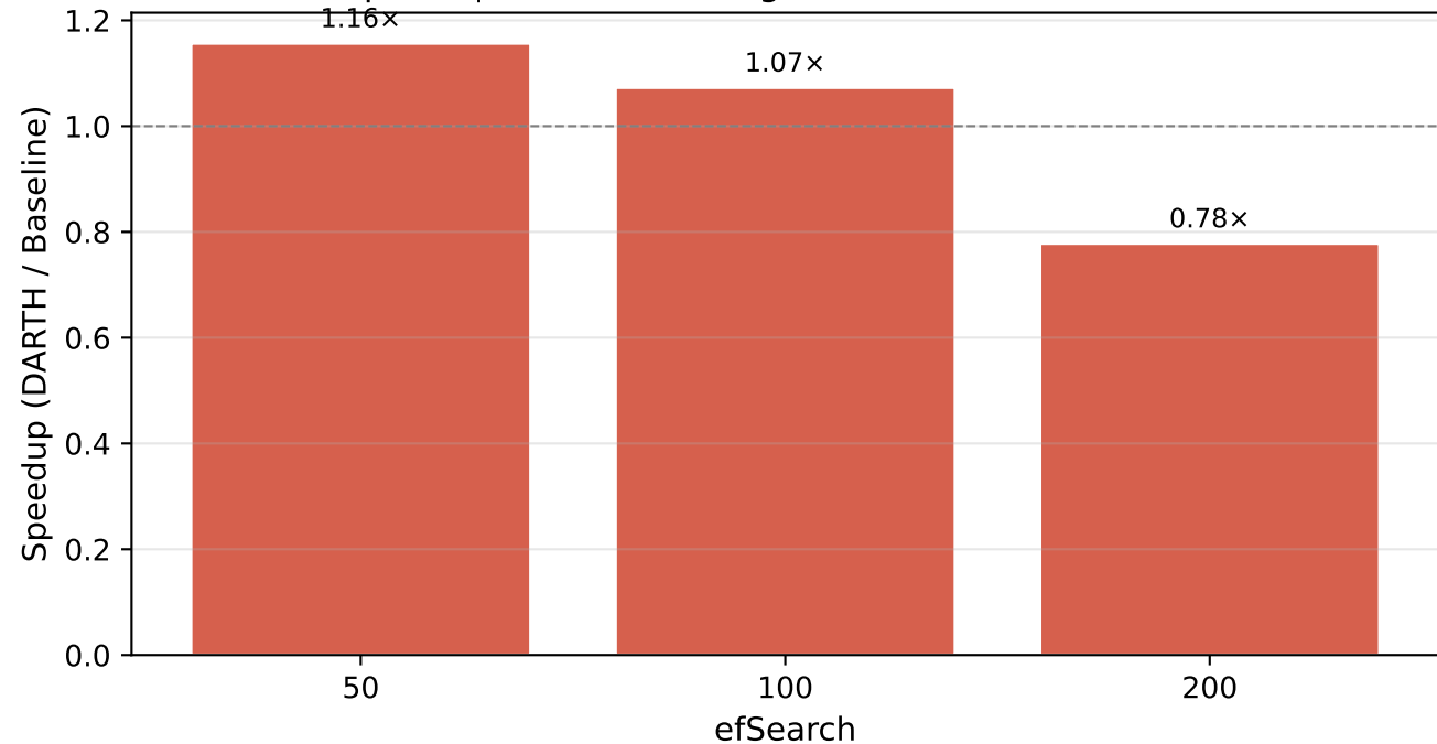
DARTH Speedup at Rt=0.90 — glove100 (M=16, efC=200, k=10)
