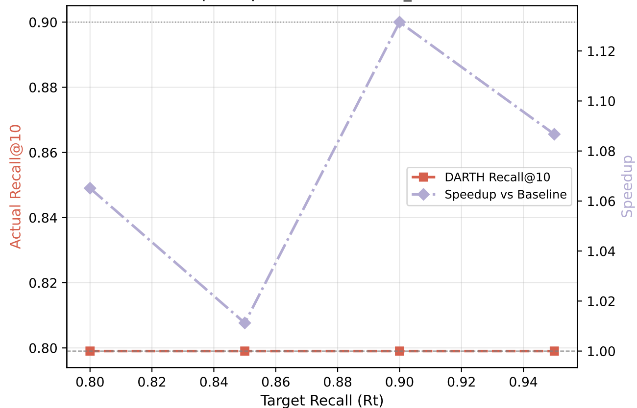
DARTH: Recall & Speedup vs Rt — msmarco_text (M=16, efC=200)
