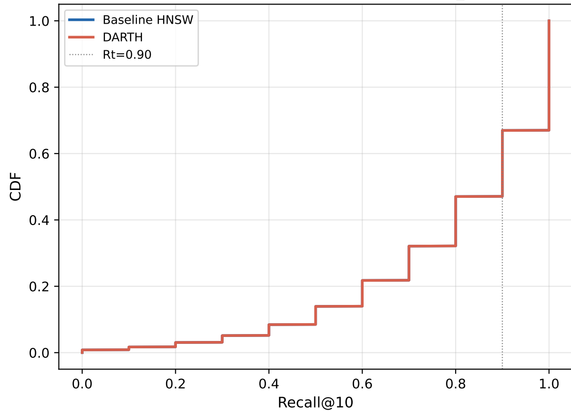
CDF of per-query Recall@10 — msmarco_text
