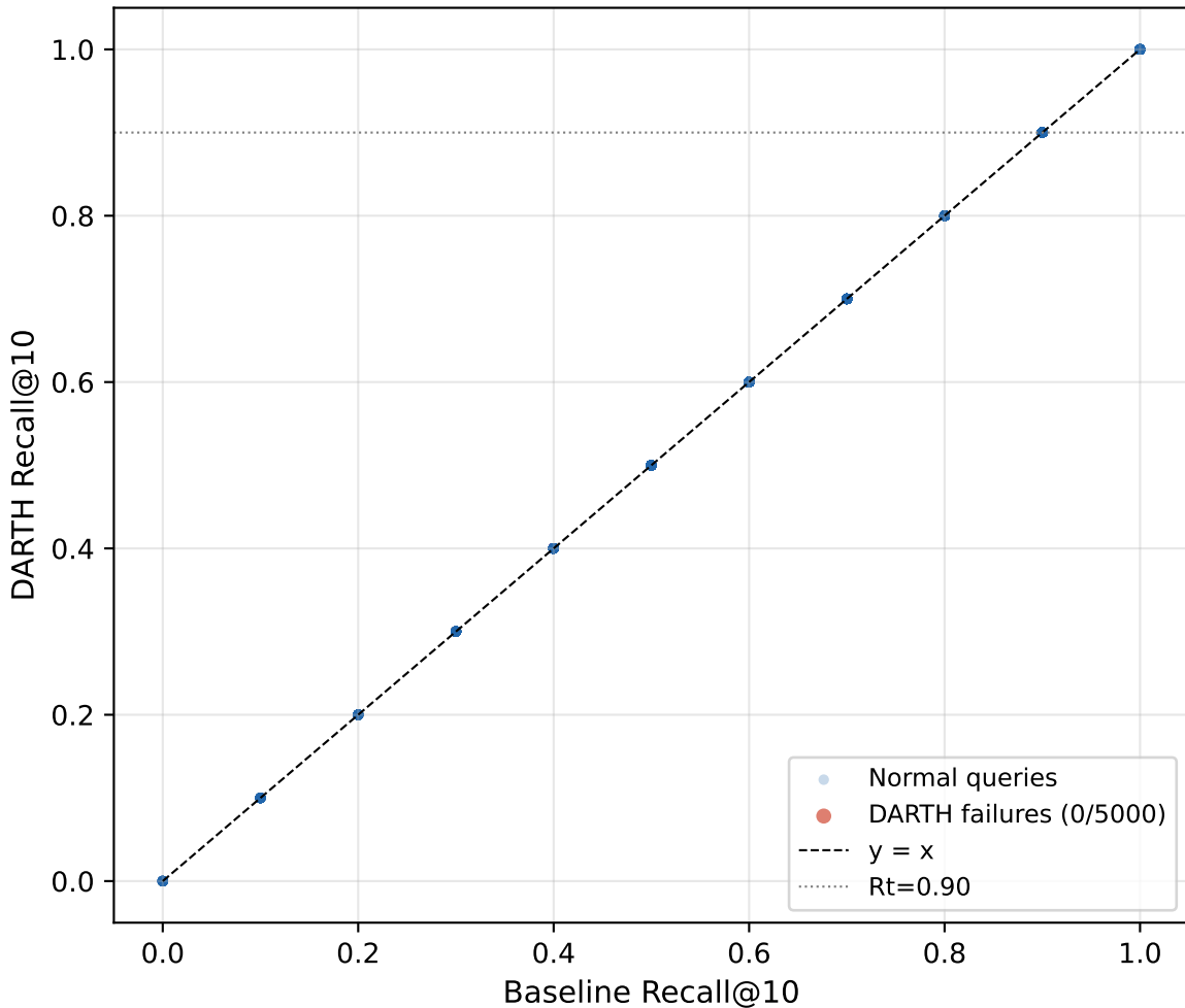
Per-query recall: Baseline vs DARTH — msmarco_text
