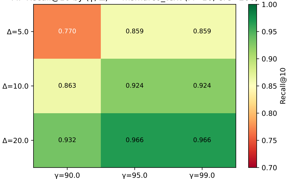
PiP Recall@10 by ( \gamma , \Delta ) — msmarco_text (M=16, efC=200)
